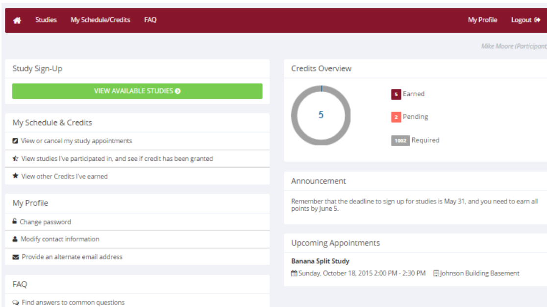
Figure 3 - Main Menu
