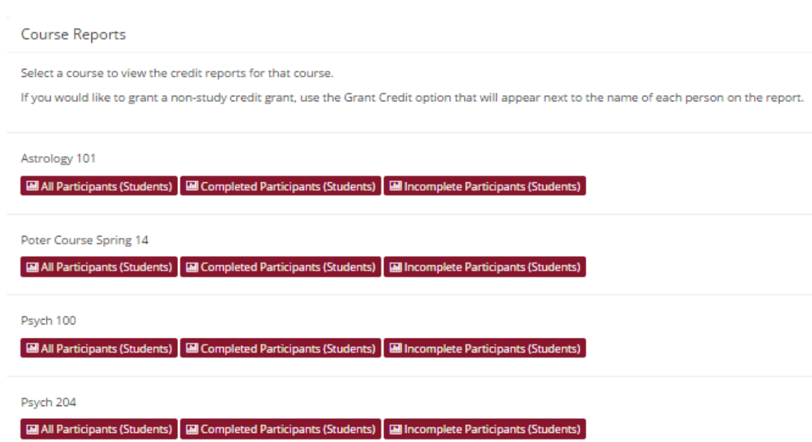
Figure 38 - Course Listing
